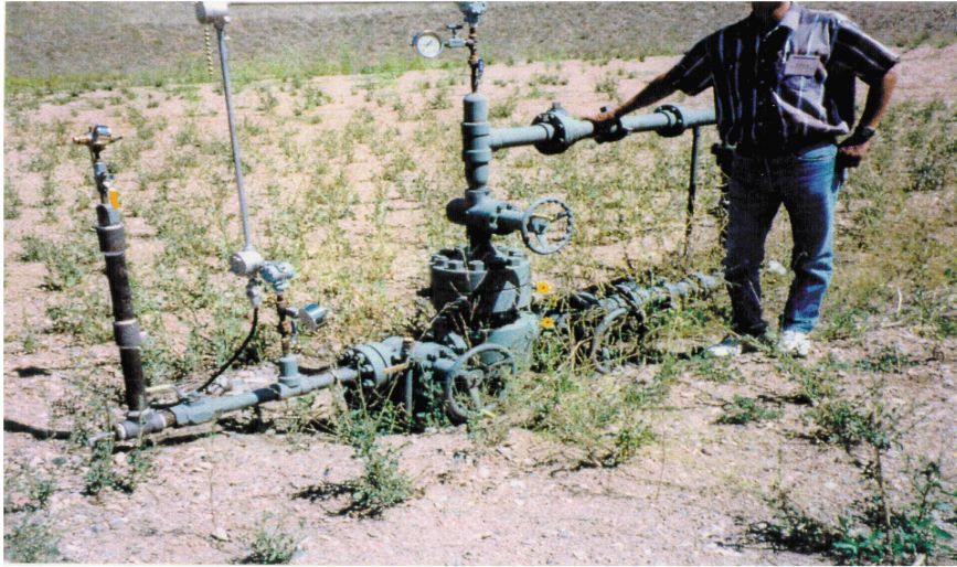
Photo 3-1 Typical Well Head
